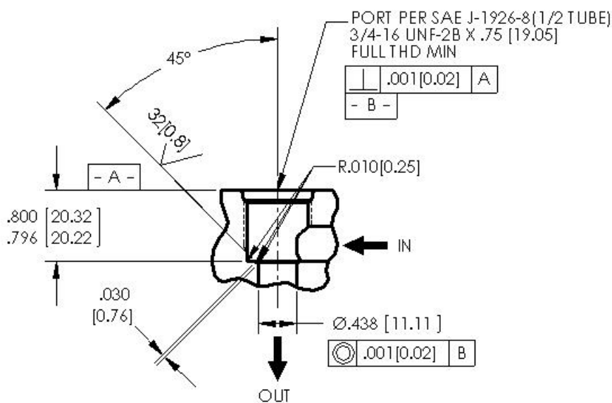
Mating Valve Seat Details
