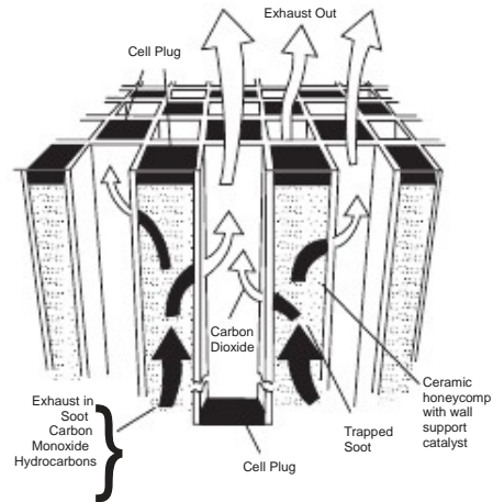
Figure 2: CPF Element (Flow rotated 90° from Figure 1)
